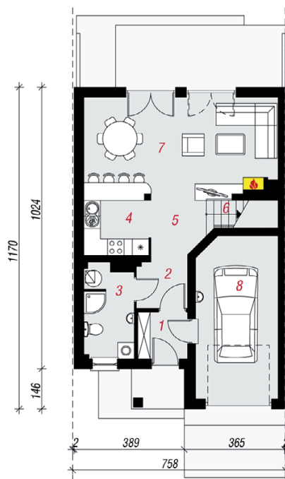
PARTER
