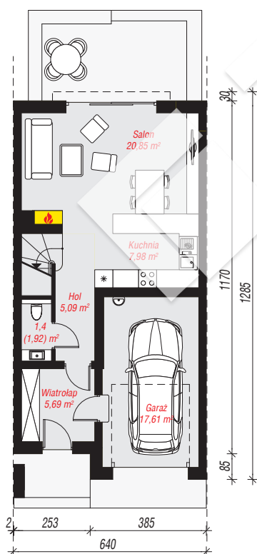
PARTER: 58,62 (59,14) m 2
