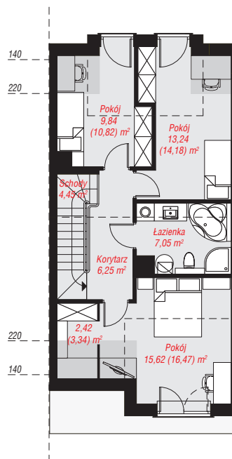
PODDASZE: 58,87 (62,56) m 2
