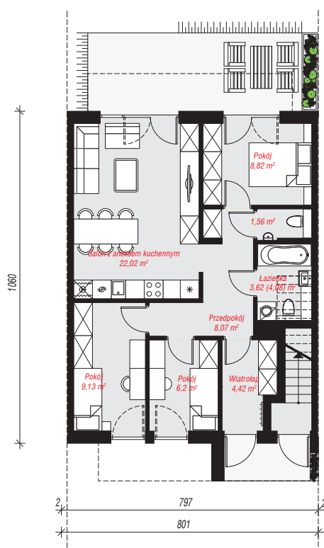
PARTER: 63,84 (64,30) m 2
