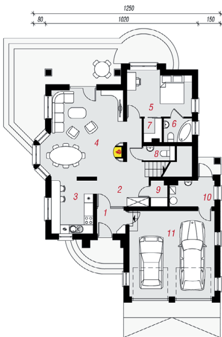
PARTER
